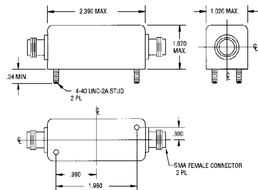
6880 Connectorized Package (50Ω Terminated)
