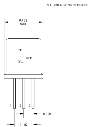
6880 F Package (2 pole F case)
