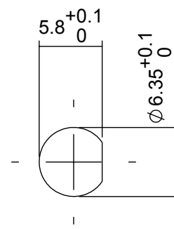
Mounting Hole
