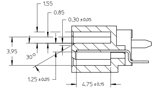
SECTION C-C
