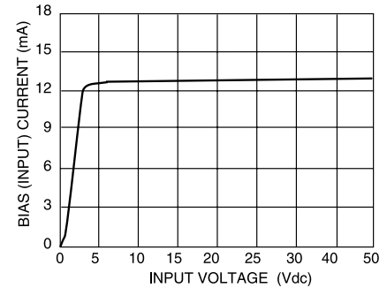
INPUT CURRENT VS INPUT VOLTAGE FIGURE 1
