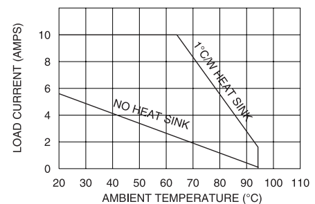
THERMAL DERATING CURVES FIGURE 3
