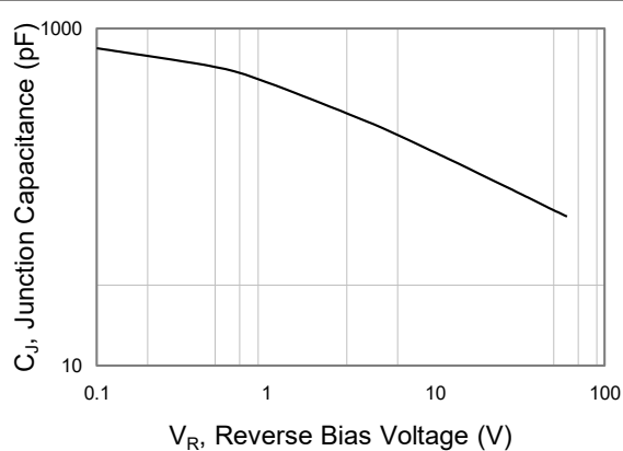
FIG. 2-TYPICAL JUNCTION CAPACITANCE
