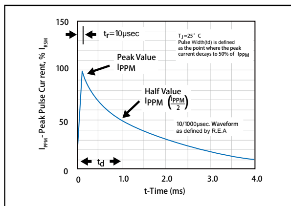
Figure 4 - Pulse Waveform
