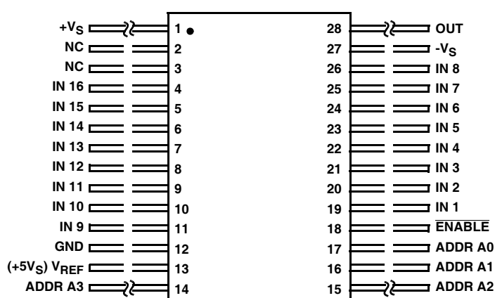
HS9-1840ARH, HS9-1840AEH, HS9-1840BRH (28 LD FLATPACK) CDFP3-F28 TOP VIEW
