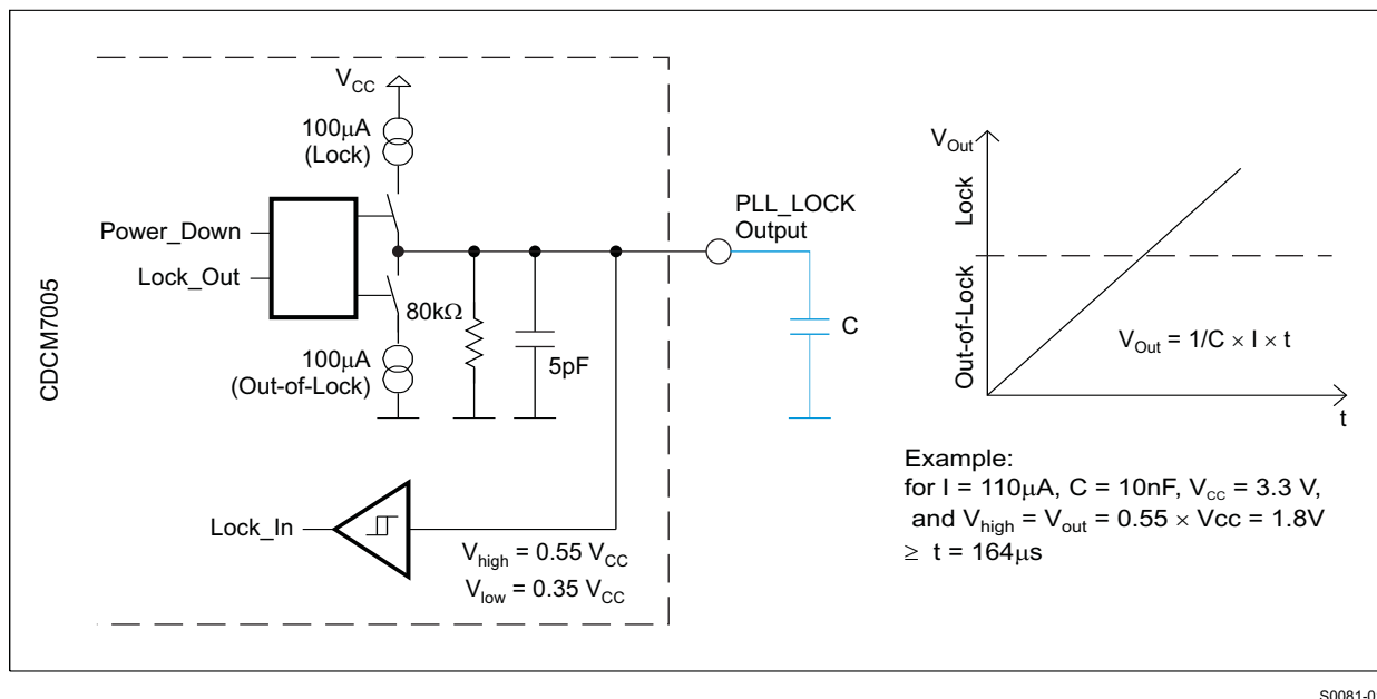
Figure 19. Analog Lock-Detect
