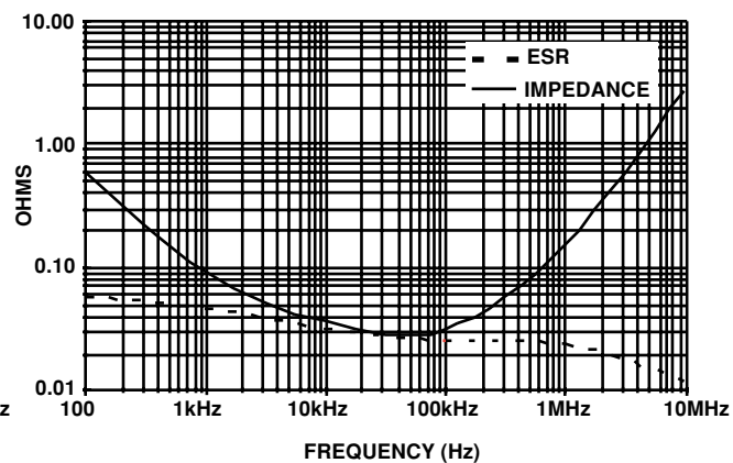
592D 2200-4V Y CASE ESR/IMPEDANCE VS FREQUENCY
