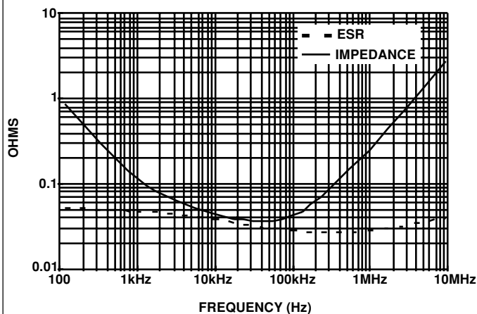
592D 1500-4V X CASE ESR/IMPEDANCE VS FREQUENCY
