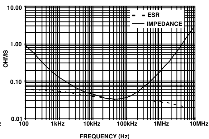
592D 1500-6.3V Y CASE ESR/IMPEDANCE VS FREQUENCY
