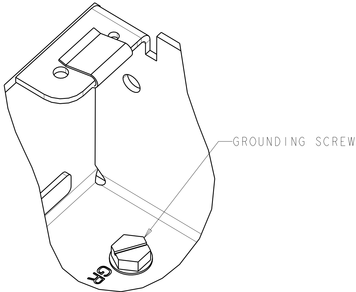
GROUNDING SCREW INSTALLATION
