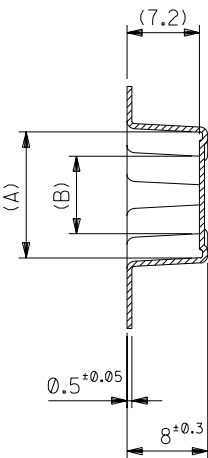
SECT. Y-Y
