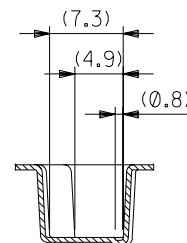
SECT. X-X
