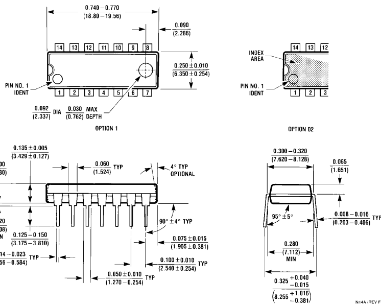
14-Lead Molded Dual-In-Line Package (N) Order Number DM7486N NS Package Number N14A
