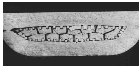
Cross Section of Insulation Piercing Crimp
