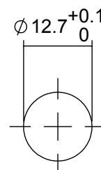
Mounting Hole
