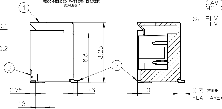
SECTION C-C
