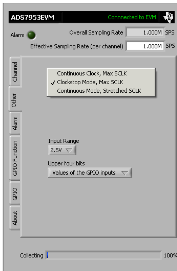
Figure 21. Serial Clock, Input Range and MS Nibble settings
