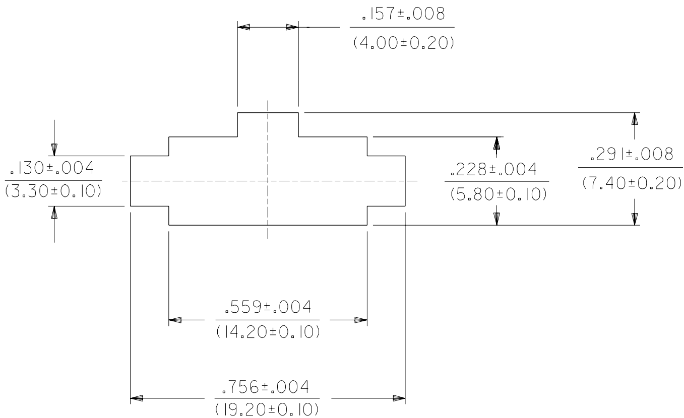
RECOMMENDED PANEL CUT-OUT (SEE NOTES 7 & 8)
