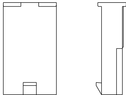
5559-03P3-*** WITHOUT MOUNTING EARS
