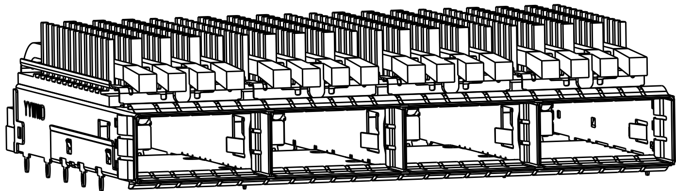
2170790-5, 5-2170790-5 AS SHOWN CUSTOMERIZED HEAT SINK SCALE 2:1
