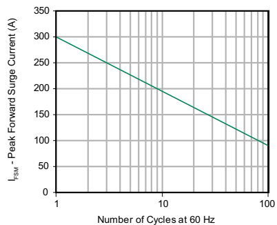
Figure 6 - Maximum Non-Repetitive Peak Forward Surge Current
