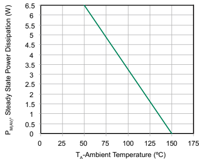
Figure 5 - Steady State Power Derating Curve
