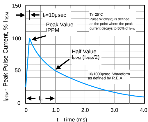
Figure 1 - Pulse Waveform
