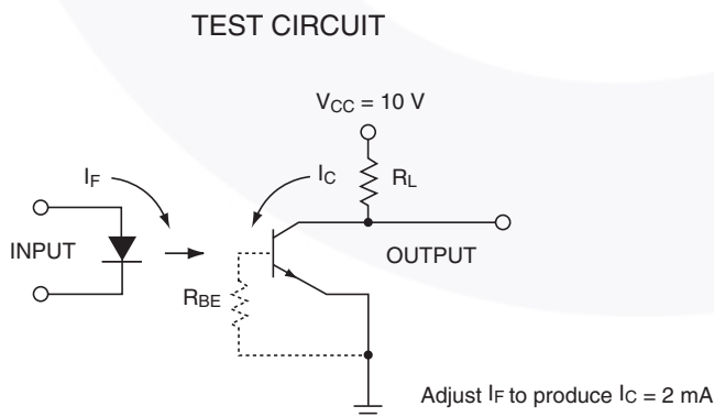
Figure 13. Switching Time Test Circuit and Waveforms
