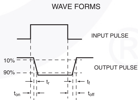
Figure 13. Switching Time Test Circuit and Waveforms
