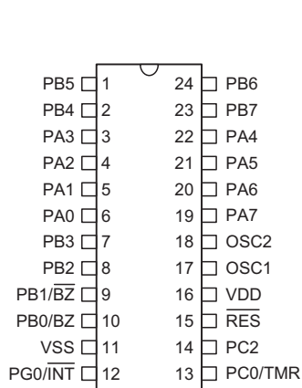
HT48E30 - 24 SKDIP-A/SOP-A
