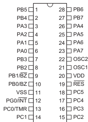
HT48E30 - 28 SKDIP-A/SOP-A
