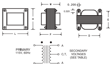
Dimensions, Inches
