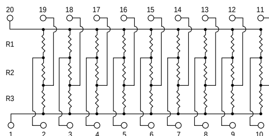
830 ELECTRICAL SCHEMATIC
