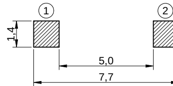
P.C.B. MOUNTING PLAN
