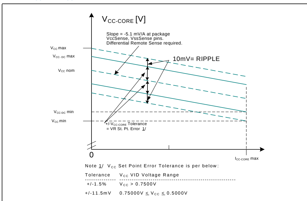
Figure 4. Active V_{CC} and I_{CC} Loadline for the Celeron M Processor Ultra Low Voltage
