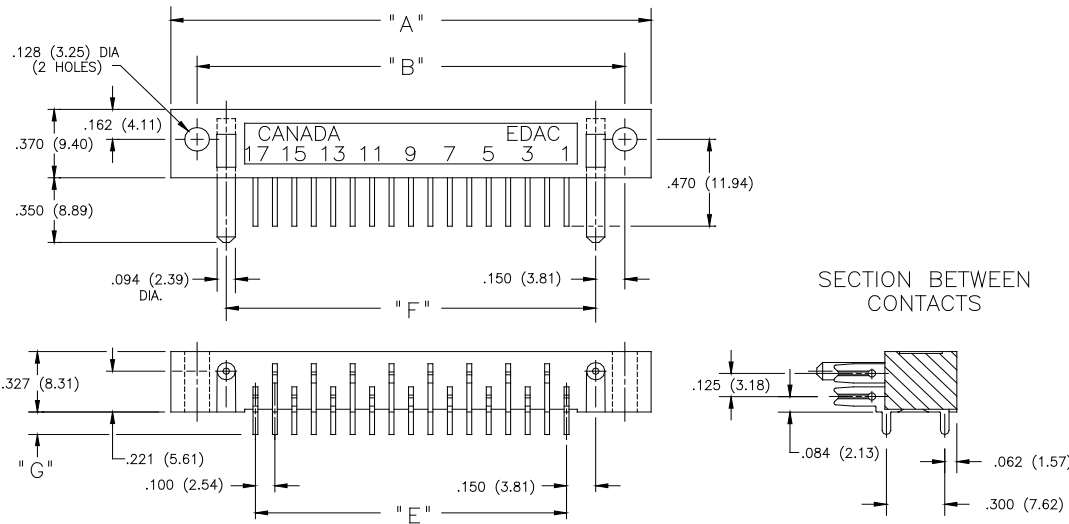
423 SERIES CONNECTOR
