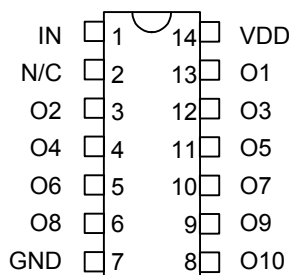
3D7010 DIP 3D7010G Gull-Wing
