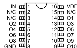
3D7010S SOL (300 Mil)
