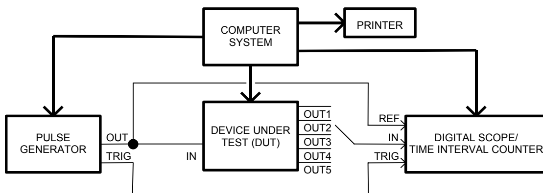
Figure 2: Test Setup
