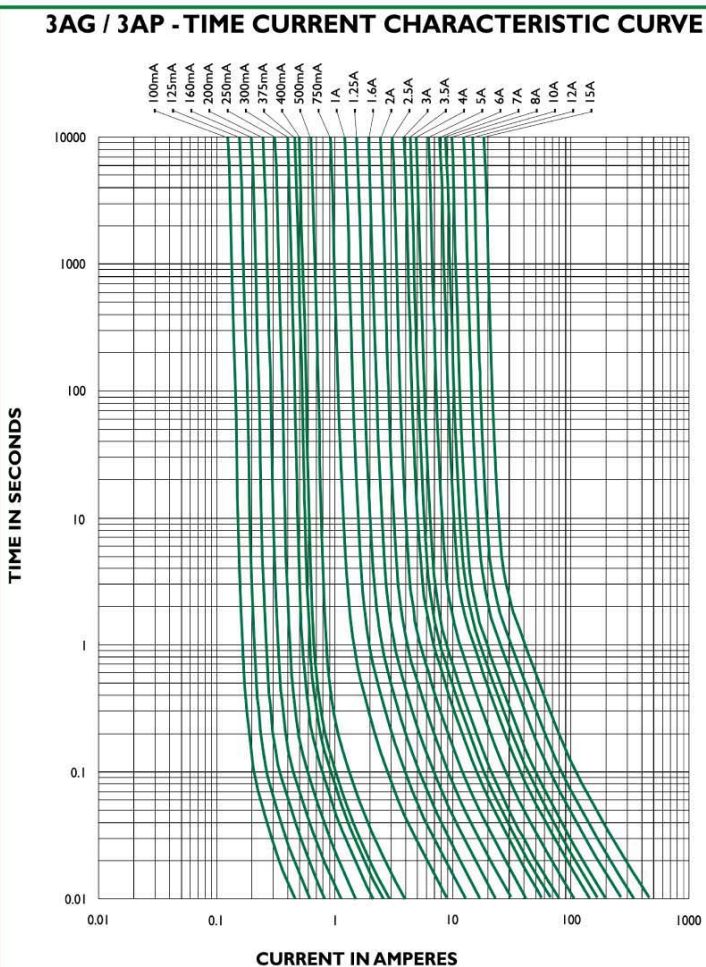
Average Time Current Curve
