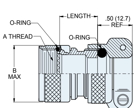
STRAIGHT ENTRY ROTATABLE COUPLING 370MS038
