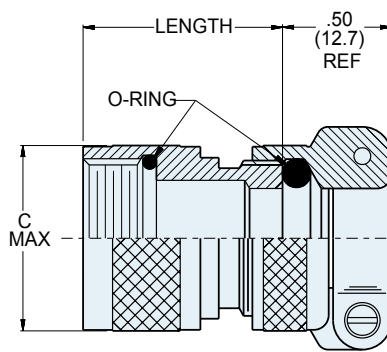
STRAIGHT ENTRY DIRECT COUPLING 370MS037
