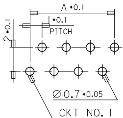
P.C. BOARD LAYOUT (MOUNTING SIDE) (THK. : 1.6t)
