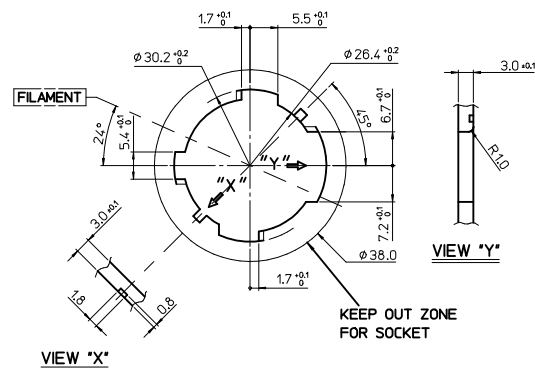
MOUNTING INTERFACE (M|-4)
