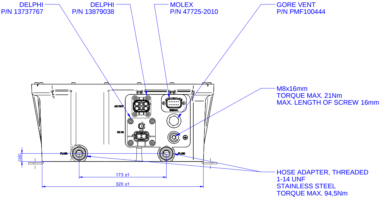
Mechanical Drawing – Front View
