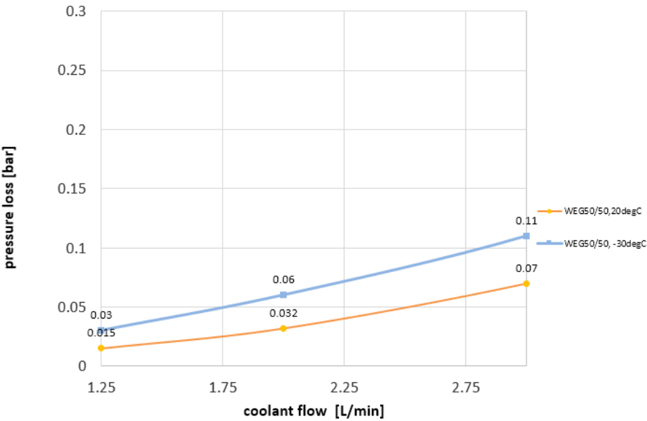
350INV60-120-240-9G Pressure losses at coolant flow dependency
