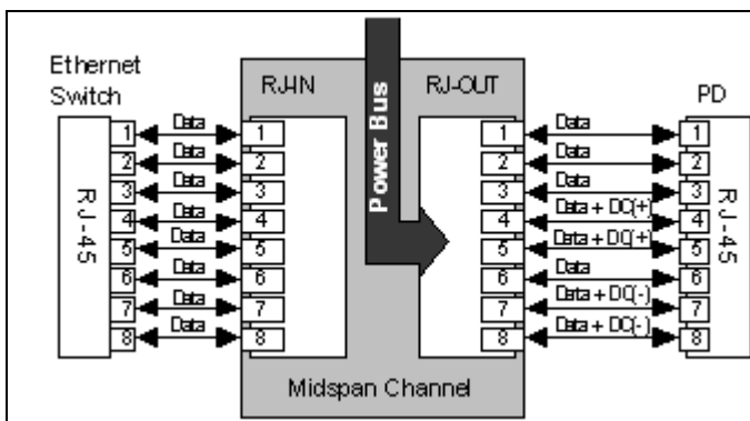
Figure 3-2: Connecting to the Midspan
