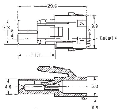
Section X-X
