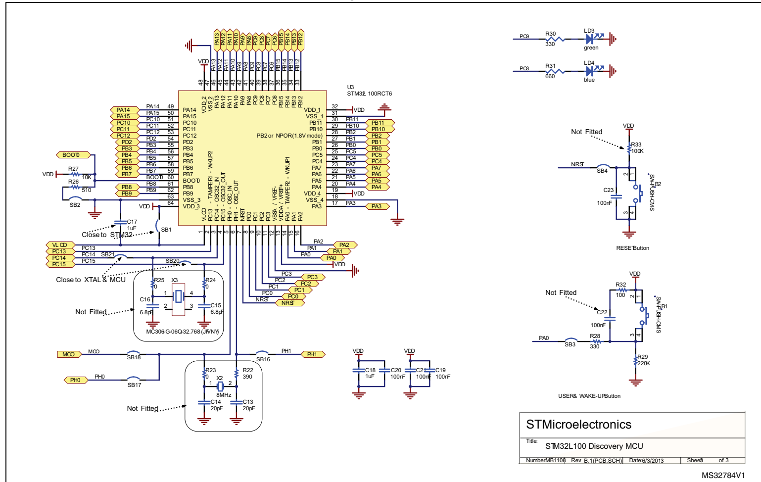
Figure 13. MCU
