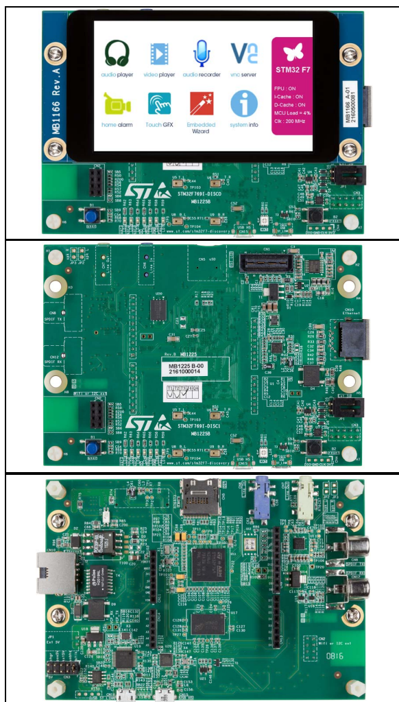
1. Pictures are not contractual. From top to bottom: STM32F769I-DISCO top view, STM32F769I-DISCO1 top view, STM32F769I-DISCO and STM32F769I-DISCO1 bottom view.
