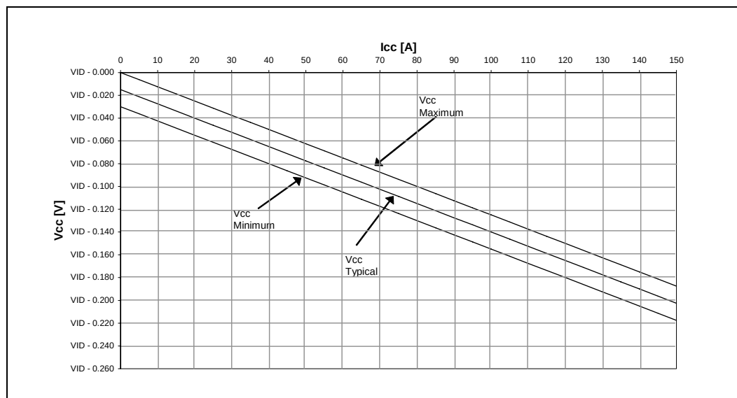
Figure 2-4. V_{CC} Static and Transient Tolerance Load Lines
