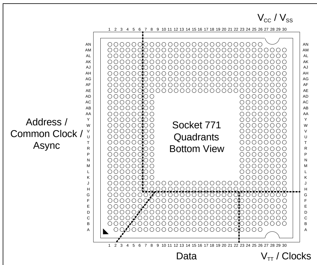
Figure 3-8. Processor Land Coordinates, Bottom View
