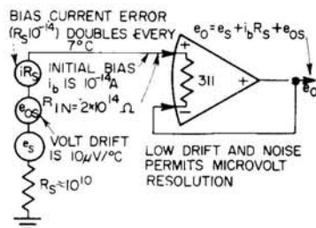
Ultra High Impedance Buffer
