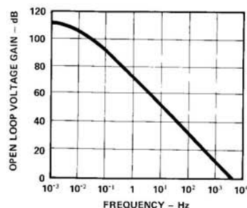
Frequency Response
