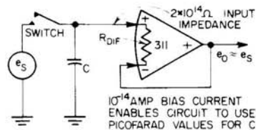
Low Capacitance Sample-and-Hold Amplifier
