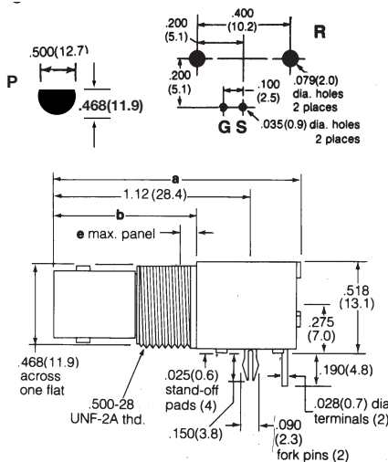
Isolated from Panel White Valox Housing 31-5486▲ (Round Pins) 31-5486-1010 (Fork Pins) 31-5486-10RFX
