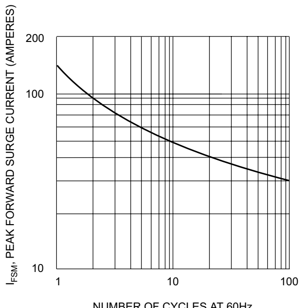
Fig. 4, Maximum Non-Repetitive Surge Current
