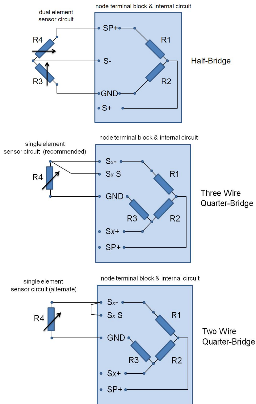
Figure 34 - Half and Quarter-Bridge Wiring
