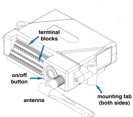
Figure 2 - Interface and Indicators
