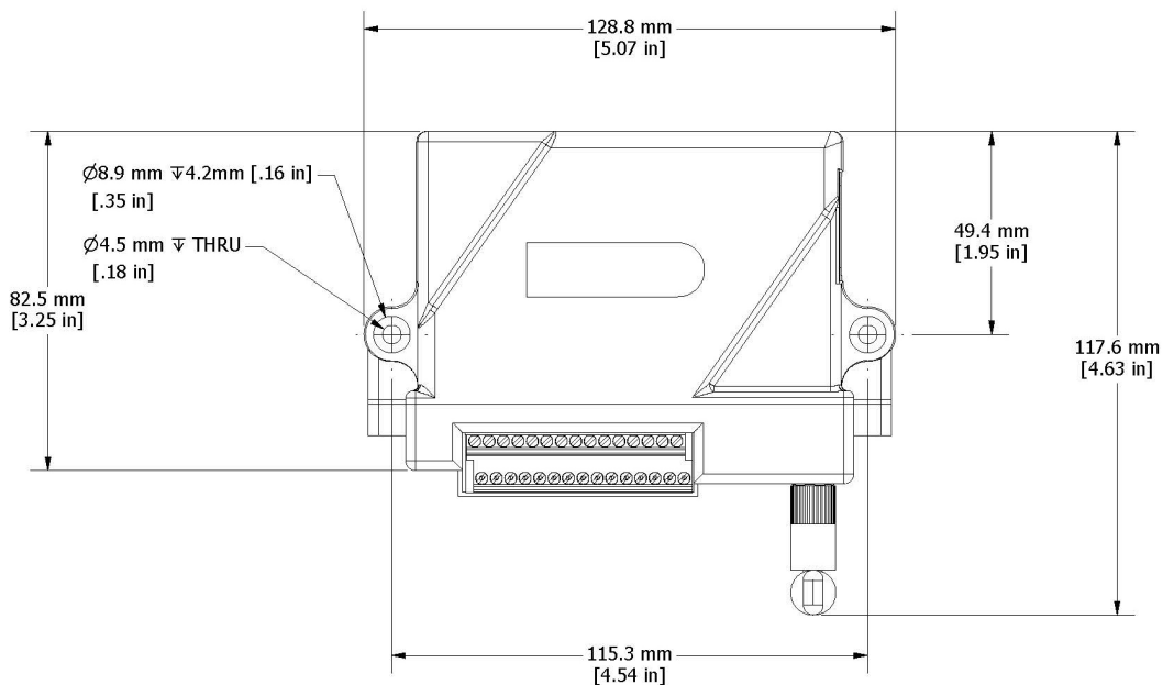
Figure 27 - Mounting the Node
