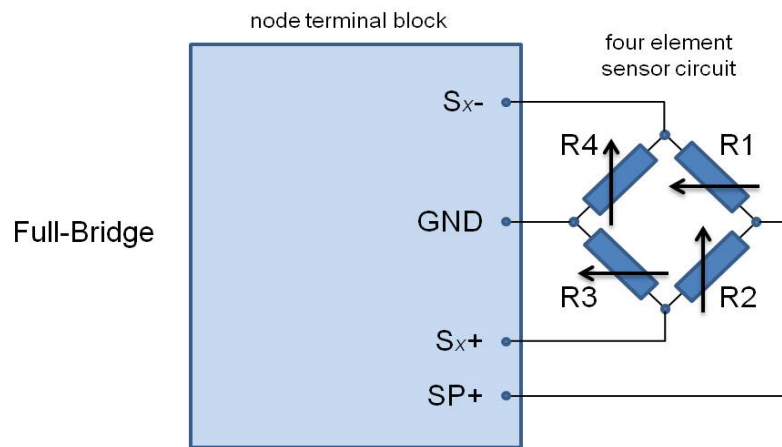
Figure 33 - Full Bridge Wiring
