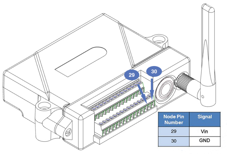
Figure 52 - External Power Connection
