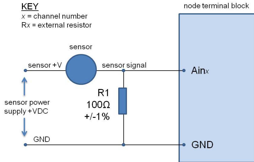
Figure 37 - Small Current Measurements
