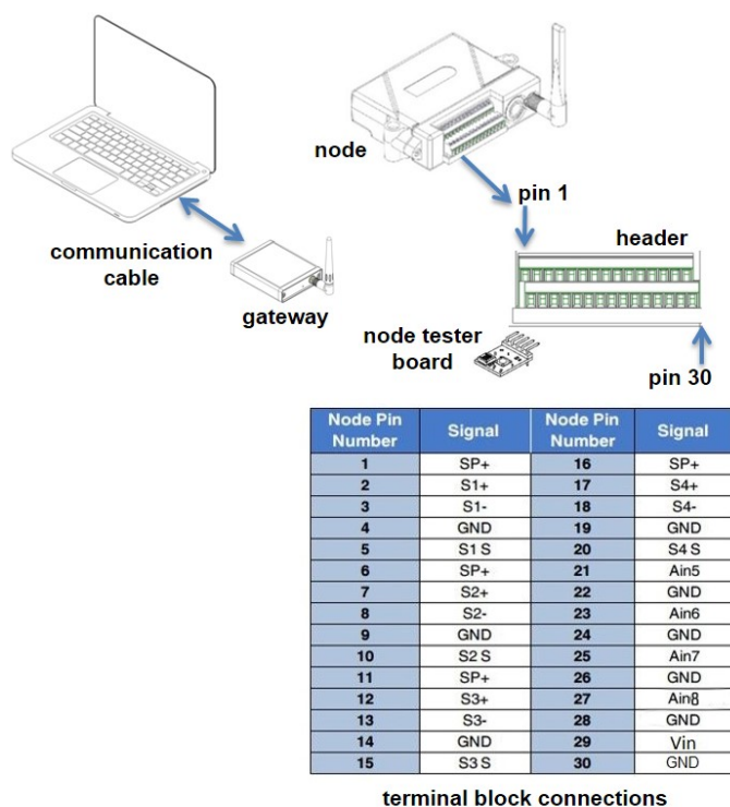
Figure 6 - System Connections
