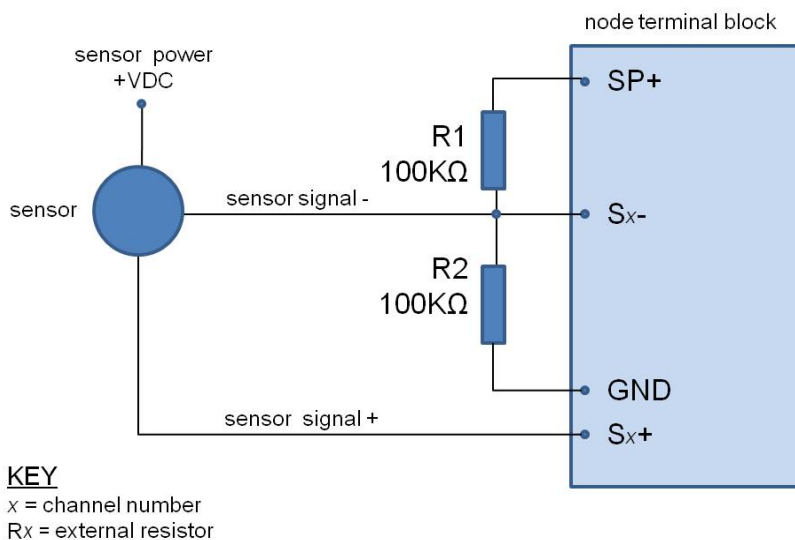
Figure 35 - Small Voltage Measurement
