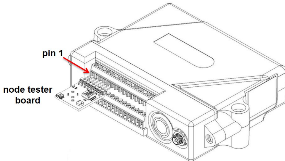
Figure 53 - Node Tester Board Installation
