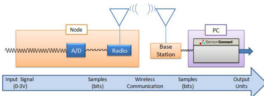
Figure 36 - Single Ended Signal Processing
