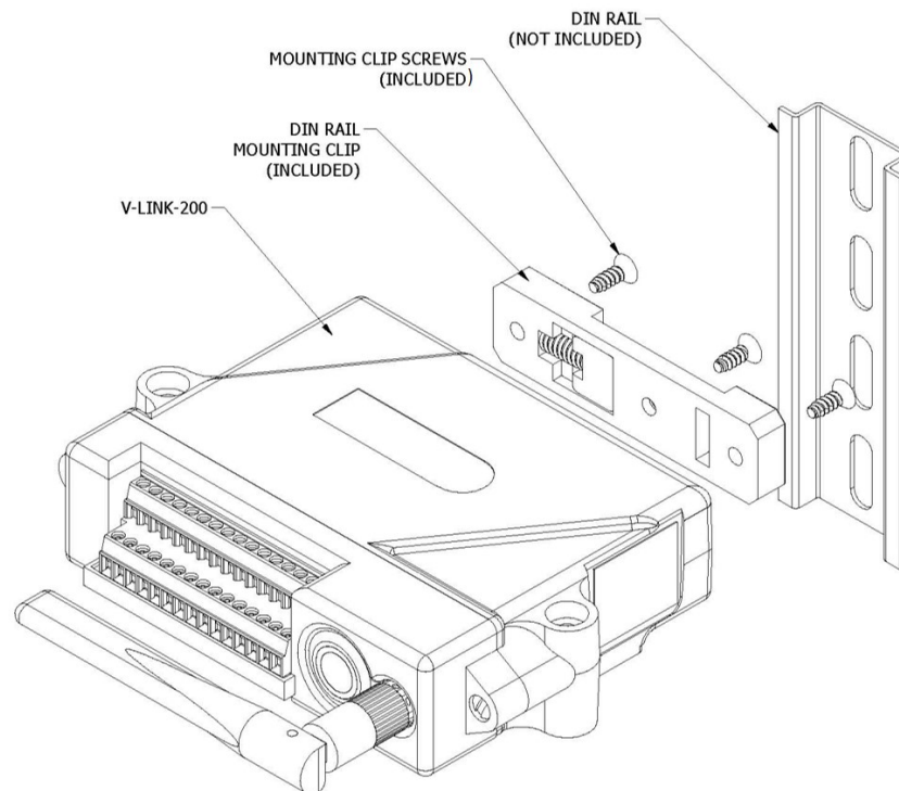
Figure 29 - DIN Rail Mount Option
