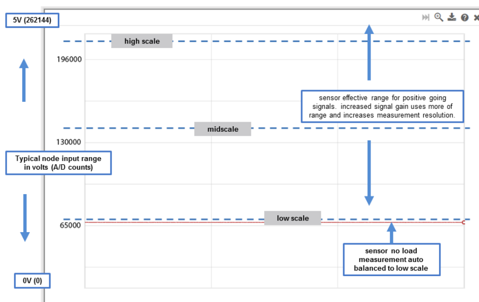
Figure 51 - Differential Input Resolution and Offset (18-bit Node)
