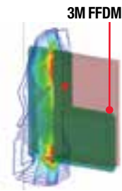
Antenna with 3M FFDM between the antenna and metal/battery parts. EM field strength increased significantly with 3M FFDM use.
