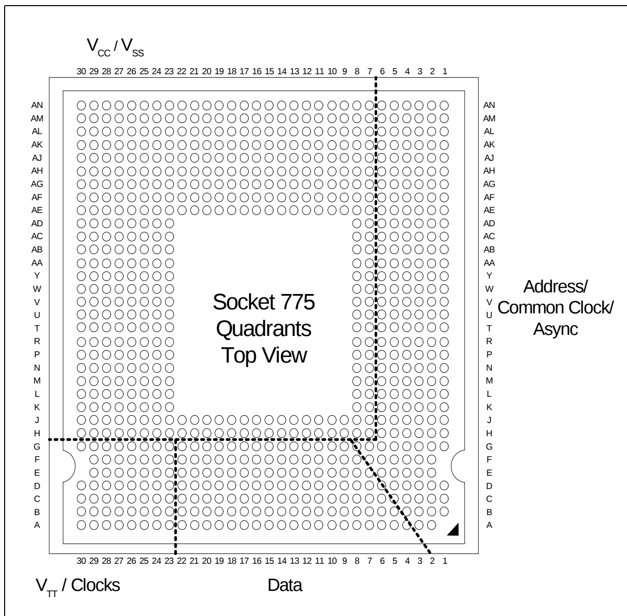
Figure 3-8. Processor Land Coordinates and Quadrants (Top View)
