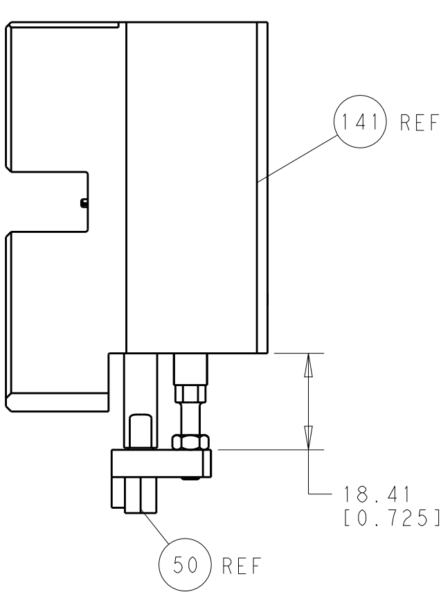
HOLDDOWN SET-UP
