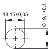
Drilling diagram
