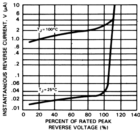
FIG.3-TYPICAL REVERSE CHARACTERISTICS
