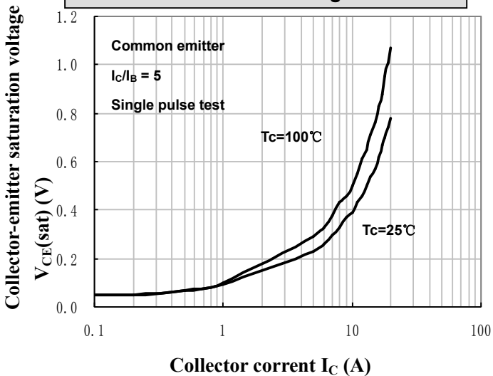
Saturation Voltage
