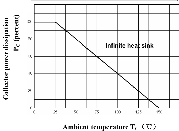
Power Derating
