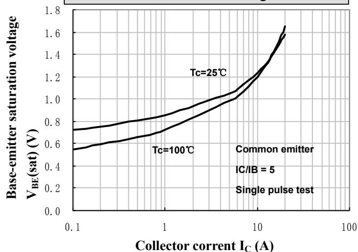
Base-Emitter Voltage
