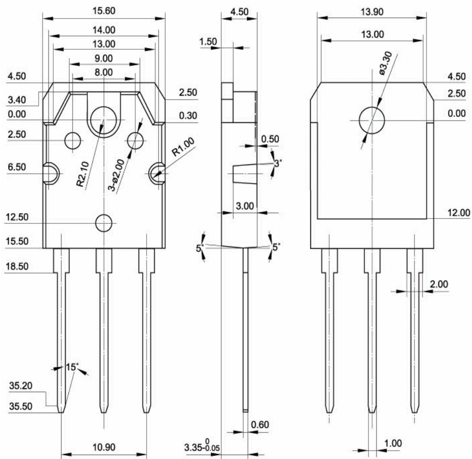
Fig.2 Outline dimensions
